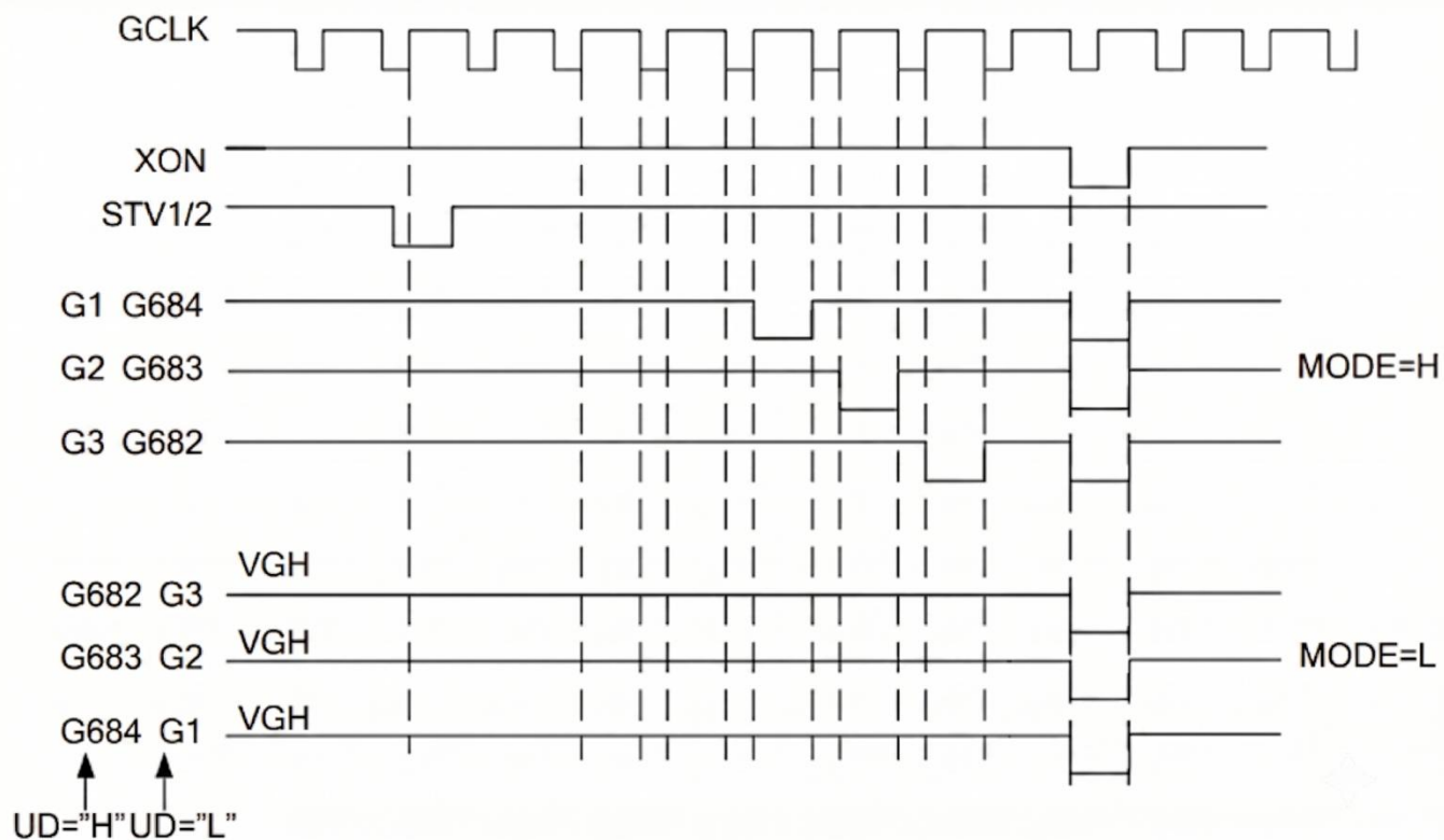
Figure: Example of input /output timing
